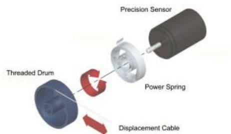
Figure 1 - How they work
